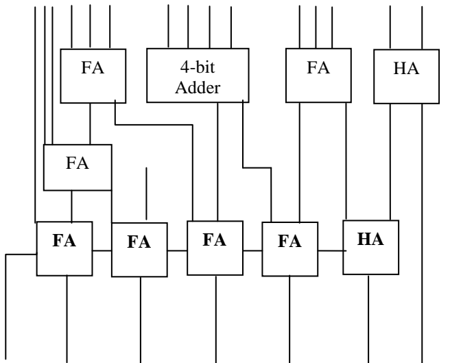
Figure 4: Block Diagram of 4-bit Multiplier using 4-bit Adder
