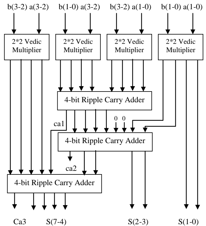
Figure 5: Block Diagram of 4-bit Vedic Multiplier
