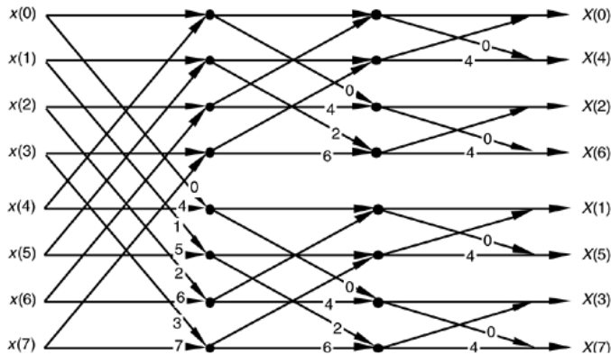
Figure 1: Radix-2 Decimation in Frequency Domain FFT Algorithm
